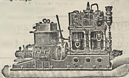
Enclosed Compound Engine and TYNE dynamo.
