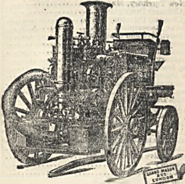
S. M. & Co.'s Improved "Double Vertical" Steam Fire Engine, constructed for the London County Council, Council of India, etc.
