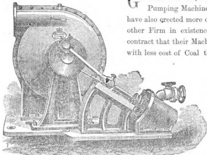
Patent Portable Pumping Engine, with Pump fixed to Engine—made in all Sizes.
